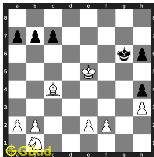
Figure 3: Initial board position of medium chess puzzle 0091
