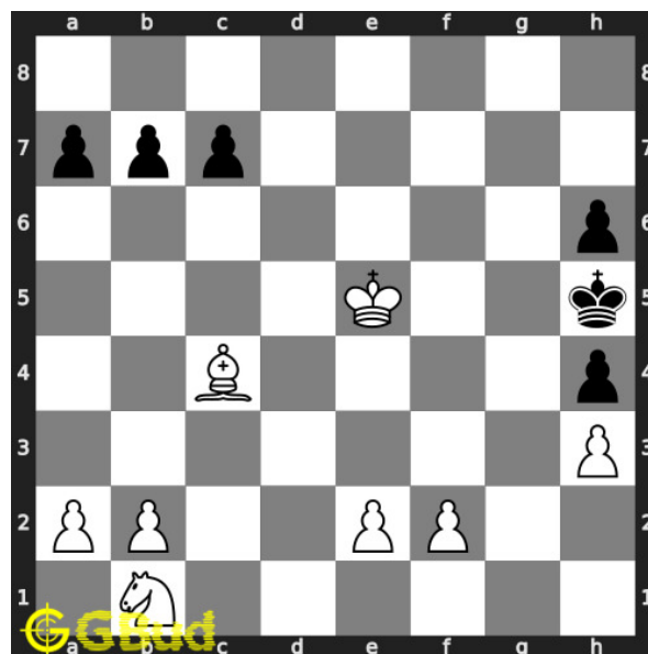
Figure 1: Solve this medium chess puzzle 0091. Mate in 2 moves @ https://gbud.in/gz7rg12
