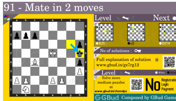
Figure 11: medium chess puzzle 91 chart 4
