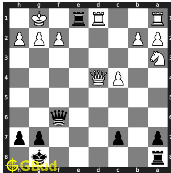
Figure 4: Re1+ - This is a deflection sacrifice and zugzwang move to force the rook to leave d1 where it is supporting the queen
